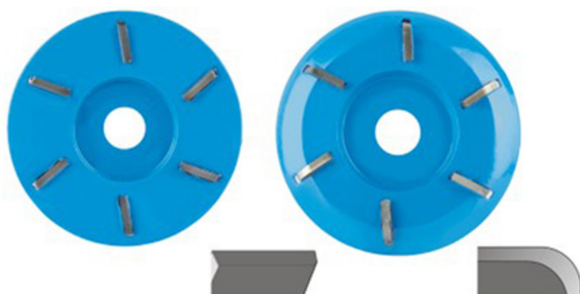
CG-D003-1 茶盘铣刀-直角刀 TEA TRAY MILLING CUTTER -RIGHT ANGLE KNIFE
